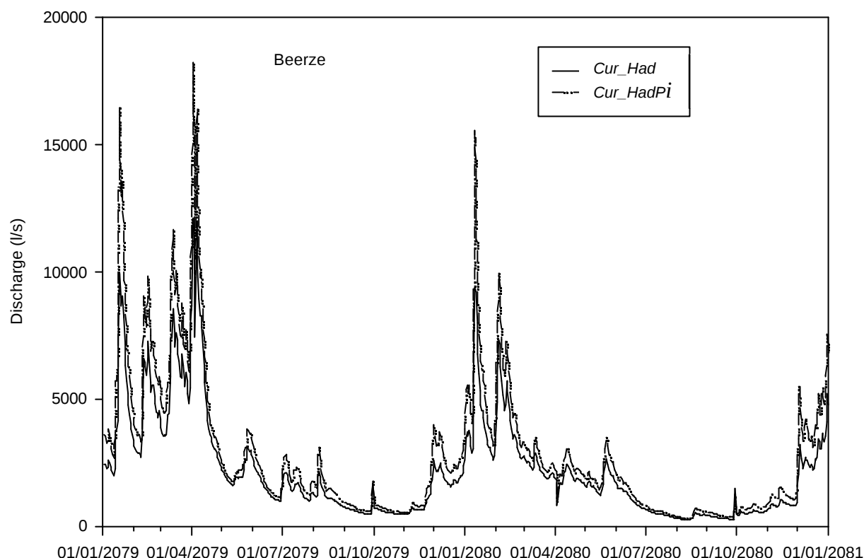
Figure 8.3 Simulated discharges of the Beerze, for scenario Cur_Had (downscaled Hadley) and Cur_HadPi with a 17% raised winter precipitation. The plotted values are daily averages of discharges computed with a time interval of 0.025 d. The sharp drop of the discharge on April 1 is due to the raising of weirs.
