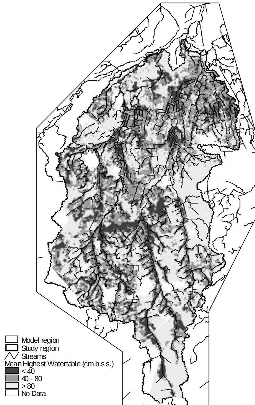
Figure 3.11 Map of the Mean Highest Watertable (final calibration).
