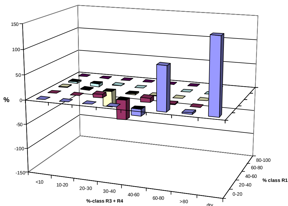
Figure 9.7 Differences between the current climate condition ( Cur_His ) and the most dynamic climate condition ( Cur_HadPi ) in percentage of sites which change of discharge dynamics class between both scenarios.
