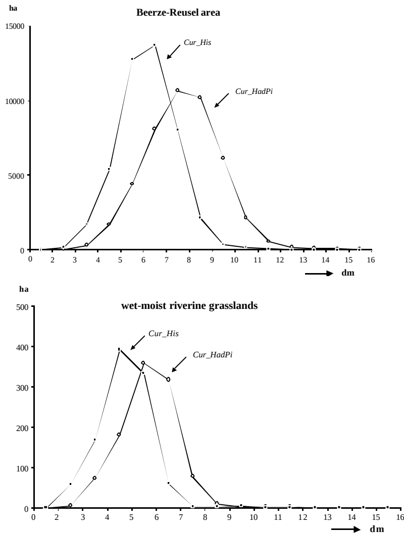
Figure 9.13 Groundwater fluctuation (difference between Mean Spring Watertable and Mean Lowest Watertable) in the current climate and in the climate scenario Cur_HadPi . Hectares per groundwater fluctuation class. Above: groundwater fluctuations in the whole study area. Below: groundwater fluctuations in wet and moist riverine grasslands only.
